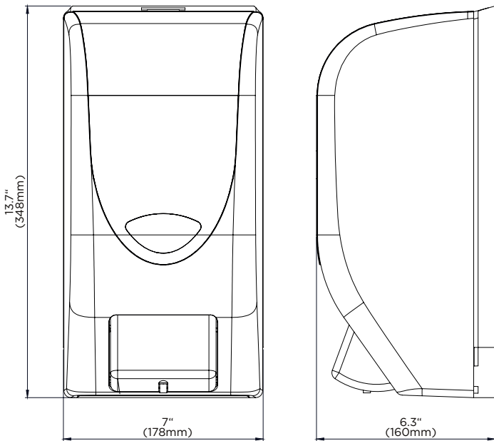
4 LITER MANUAL DISPENSER
