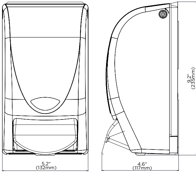
1 LITER MANUAL DISPENSER
