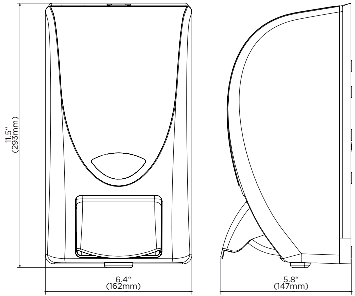
2 LITER MANUAL DISPENSER
